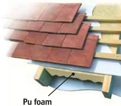
Pitched roof, ceiling at rafter line
